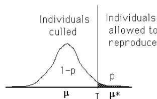
Figure 5.1. Under truncation selection, the uppermost (or lowermost) fraction p of a population is selected to reproduce. Alternatively, one could set a threshold level in advance, above (below) which individuals are allowed to reproduce. To predict response given either p or T , we need to know the mean of the selected tail ( \mu^* ), from which we can compute S = \mu^* - \mu and then apply the breeders' equation.
