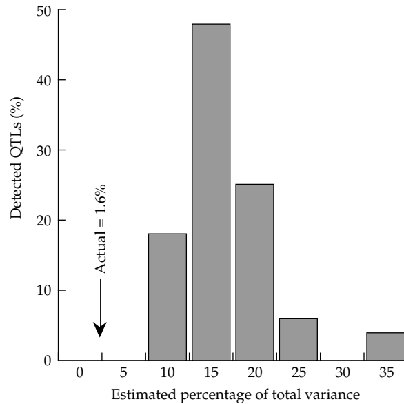
Figure 17.4 Distribution of the estimated effects of detected QTLs. Here 40 QTLs, each accounting for 1.58% of the variance, are assumed. Using 100 F_2 individuals, only 4% of such loci were detected. The average estimated fraction of total variation fraction accounted for by each detected QTLs was 16.3%, with the distribution of estimates skewed towards larger values. (From Beavis 1994.)
