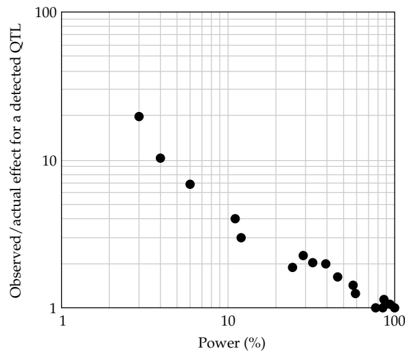
Figure 17.3 Relationship between the probability (power) of detecting a QTL and the amount by which the estimated effect of a detected QTL overestimates its actual value. (Based on Beavis 1994.)
