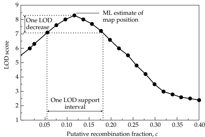
Figure 17.1 Hypothetical likelihood map for the marker-QTL recombination frequency c in a single-marker analysis. Points connected by straight lines are used to remind the reader that likelihood maps are computed by plotting the maximum of the likelihood function for each c value, usually done by considering steps of 0.01 to 0.05. A QTL is indicated if any part of the likelihood map exceeds a critical value. In such cases, the ML estimate for map position is the value of c giving the highest likelihood. Approximate confidence intervals for QTL position (one-LOD support intervals) are often constructed by including the set of all c values giving likelihoods within one LOD score of the maximum value.
